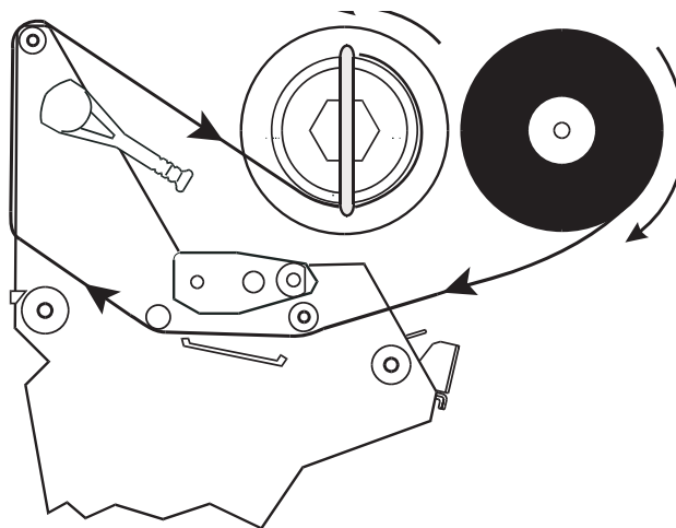
Figure 21 • Ribbon Path
